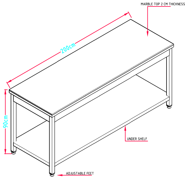
ISOMETRIC
